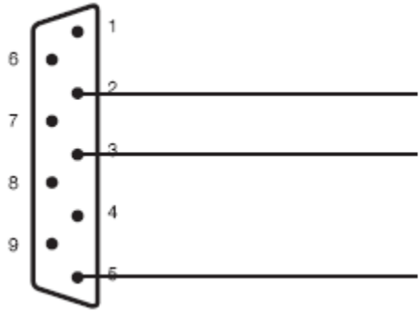
D-SUB 9pin Male
