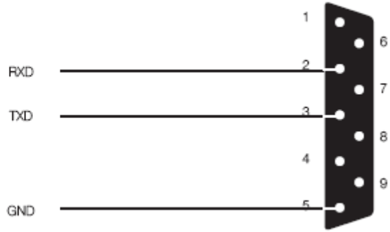
D-SUB 9pin Female
